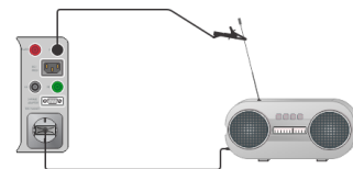
Substitute leakage test for Class II device
