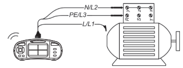
Test circuit for continuous resistance measurement
