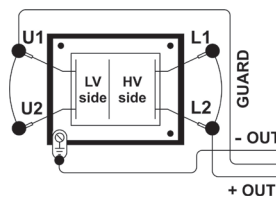
The simplest measurement of insulation resistance of transformer
