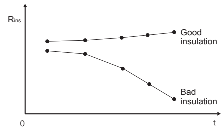
Typical step voltage measurement results
