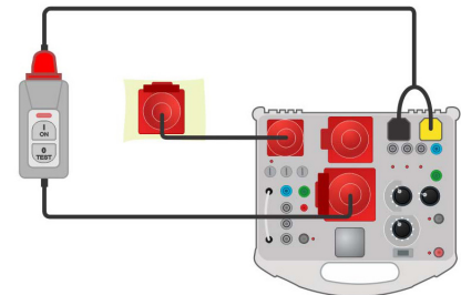
Testing the 3-phase PRCD
