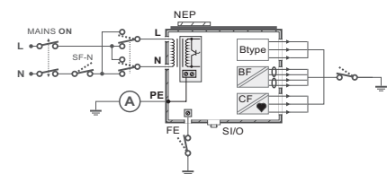
Class I Earth leakage measurement
