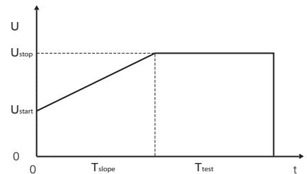
Measuring procedure for withstanding voltage measurement.
