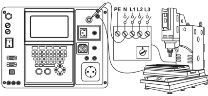
HV withstanding test
