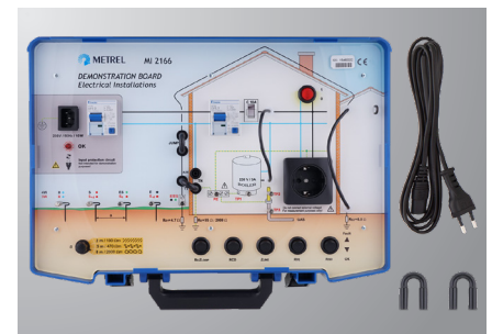
Picture of MI 2166 set
