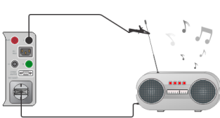
Touch leakage current test for Class II device
