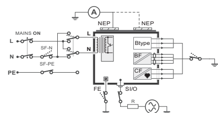
Touch current measurement
