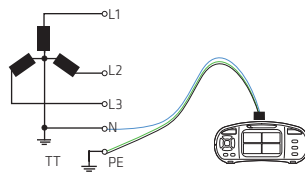
Two-wire method (test from the socket between N and PE)
