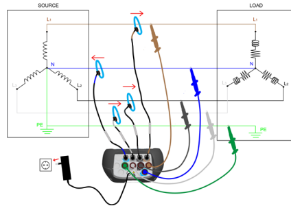
Connection to 3-phase 4-wire system
