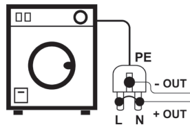
Measurement of household device, protection class I and class II
